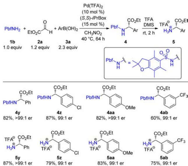
Scheme 5. Examples with Pbf-Sulfonamide and Their Deprotection a
