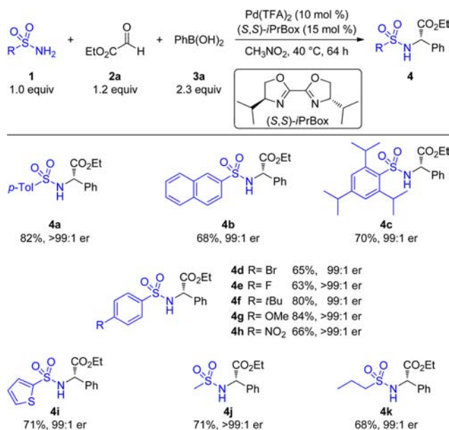
Scheme 2. Variation of Sulfonamides a
