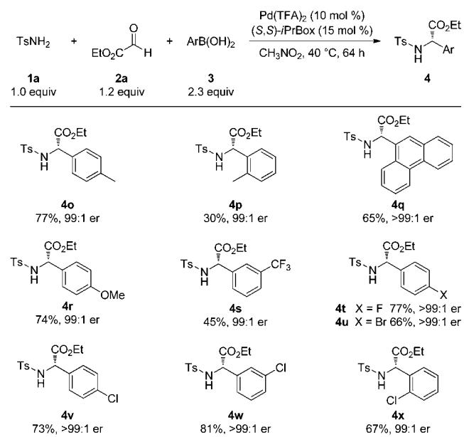
Scheme 4. Variation of Boronic Acids a
